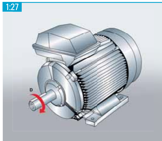
The mains supply is connected to a three-phase motor’s terminals marked U, V and W. The phase sequence is L1, L2 and L3. This means the motor will rotate clockwise seen from “D” the drive end. To make the motor rotate anticlockwise two of the three conductors connected to the starter or to the motor are switched. Check the operation of the cooling fan when rotating anticlockwise.
