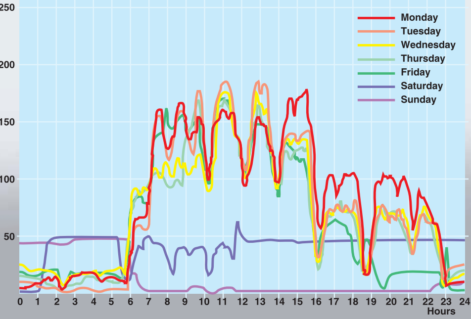
During an operation analysis the compressed air production is continuously measured for a full week.
