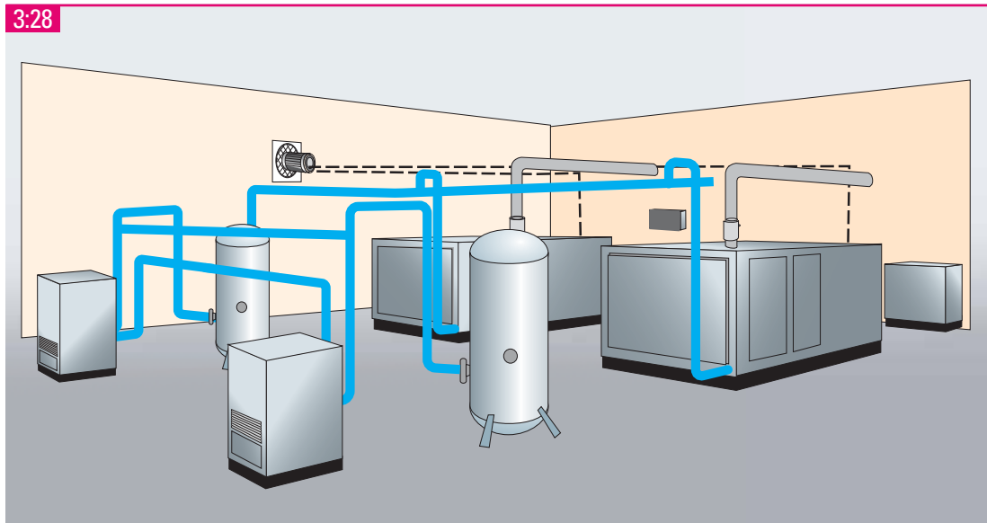
It is important that the compressor installation has a layout that is service friendly and flexible to accommodate future expansion. The minimum area at service points in front of the machine electrical cabinets should be 1200 mm.
