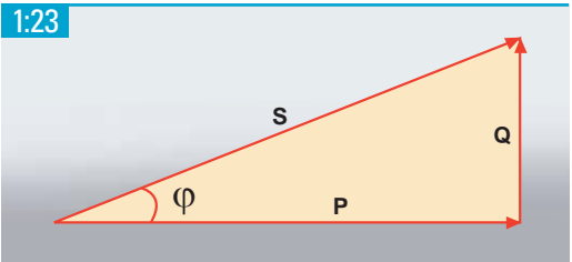
This illustrates the relation between apparent power ( S ), reactive power ( Q ) and active power ( P ). The angle \varphi between S and P gives the power factor \cos(\varphi) .
