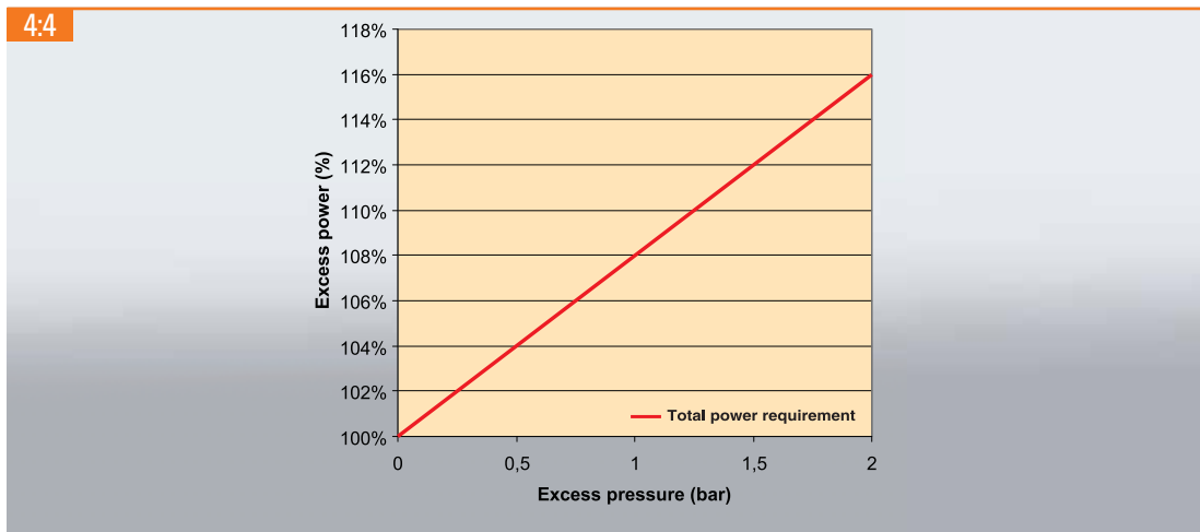
Excess power requirement as a result of over-pressurizing to compensate for pressure drops. For a 300 l/s compressor, raising the working pressure by 1 bar means 6 kW higher power consumption. At 4000 operating hours/year this represents 24,000 kWh/year or € 2,400/year.
