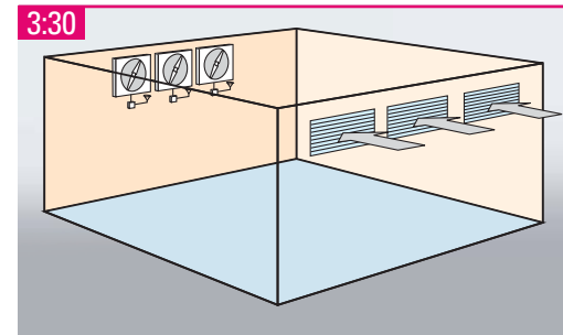
System with several thermostat-controlled fans, which together can handle the total ventilation requirement. The thermostats on the individual fans are set for different ranges, which means that the quantity of ventilation air can vary depending on the outside temperature and/or the number of compressors in use (as the thermostats will switch on the fans one after another depending on the temperature in the compressor room). Alternatively, the fans can be started via a multi-stage thermostat.
