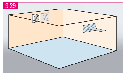
Basic ventilation solution. The disadvantage is that ventilation is constant irrespective of the outside temperature. In addition difficulties can occur if two compressors are installed. The fans will be over-dimensioned if only one of the compressors is used. The problem can be solved by fitting the fans with speed controlled motors, which start via a multi-stage thermostat.
