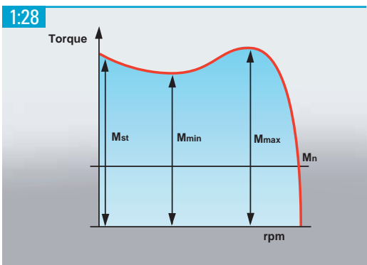
The torque curve for a squirrel cage induction motor. When the motor starts the torque is high. M_{st} = start torque, M_{max} = max torque (“cutting torque”), M_{min} = min. torque (“saddle torque”), M_n = rated torque.
