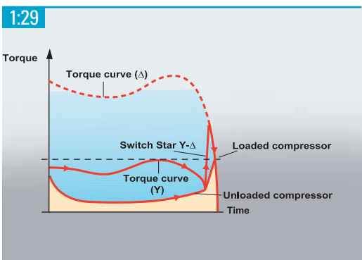
A star/delta started induction motor torque curve combined with a torque demand curve for a screw compressor. The compressor is unloaded (idling) during star operations. When the speed has reached approx. 90-95% of the rated speed the motor is switched to the delta mode, the torque increases, the compressor is loaded and finds its working point.
