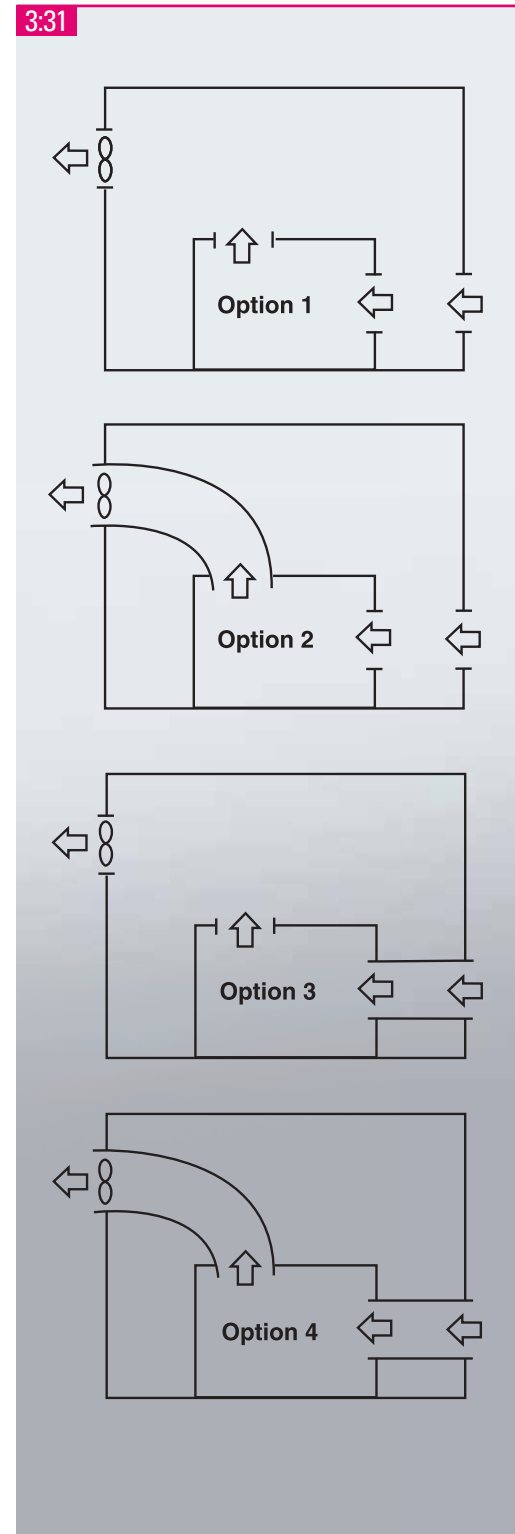
Examples of different ventilation solutions.
